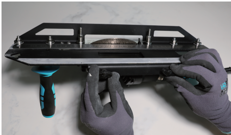
Step 2. Turn the adjusting screws in colockwise/ counterclockwise,keep both screws adjusted. Colorwise turn to get thinner cutting edge Counterclockwise to get a thicker cutting edge
